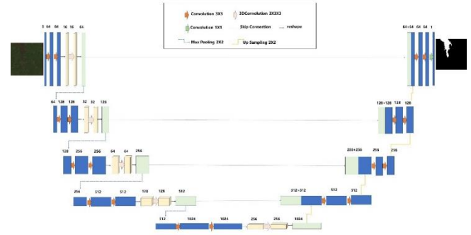
Fig. 4. Schematic of SSU-Net (adapted from [28]).
